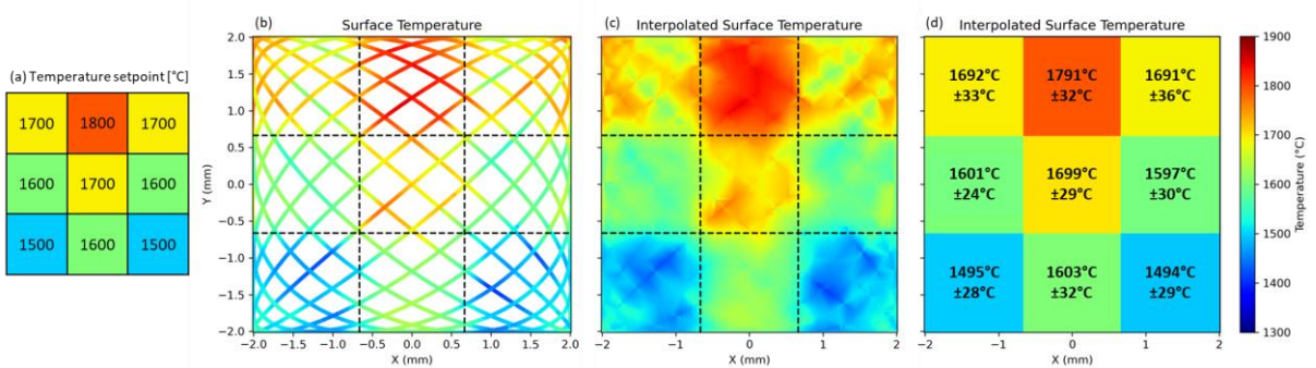
Fig. 8. Measured temperature of a steel 1.4404 sample with 3*3 temperature zones. (a) temperature setpoints; (b) temperature data along the oscillation path; (c) interpolated temperatures; (d) average temperatures with standard deviation
